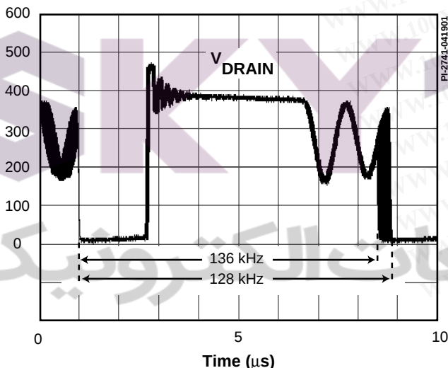
Figure 4. Frequency Jitter.
